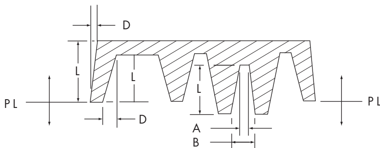
Drawing defines draft dimensions for interior and exterior surfaces and total draft for holes (draft is exaggerated for illustration).
